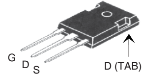
TO-247 (IXTH)
