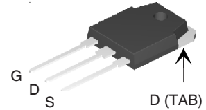
TO-3P (IXTQ)
