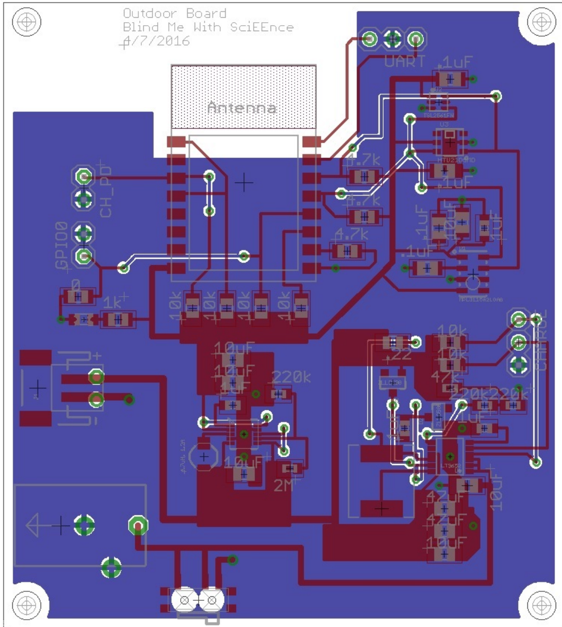
Figure 4. Outdoor Board Layout
