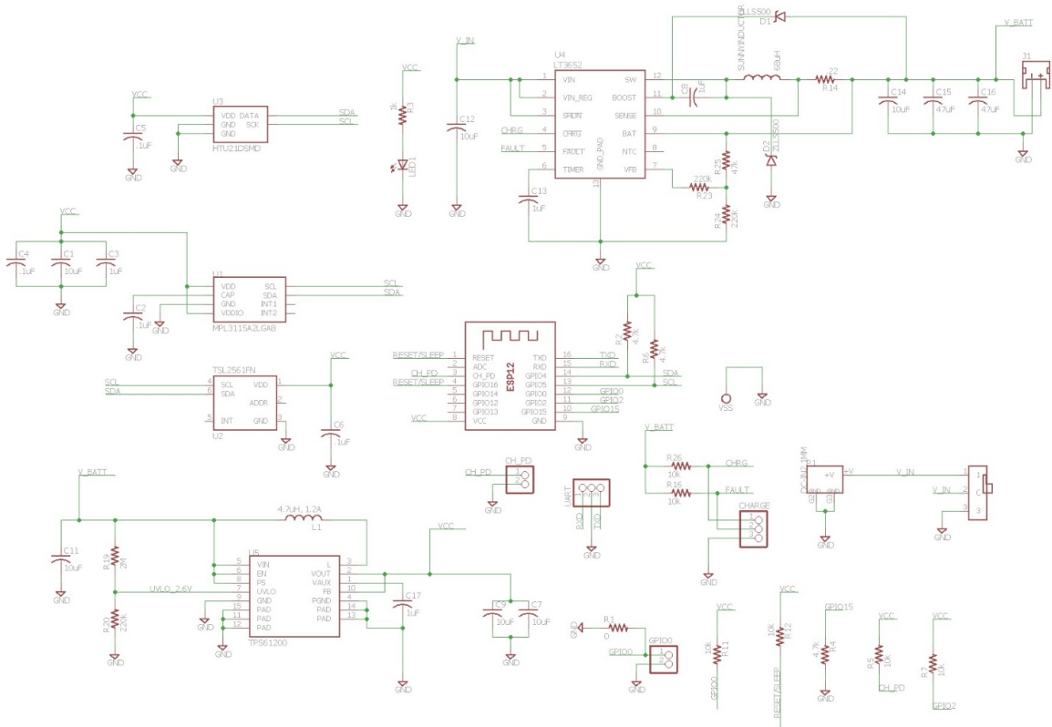
Figure 3. Outdoor Board Schematic
