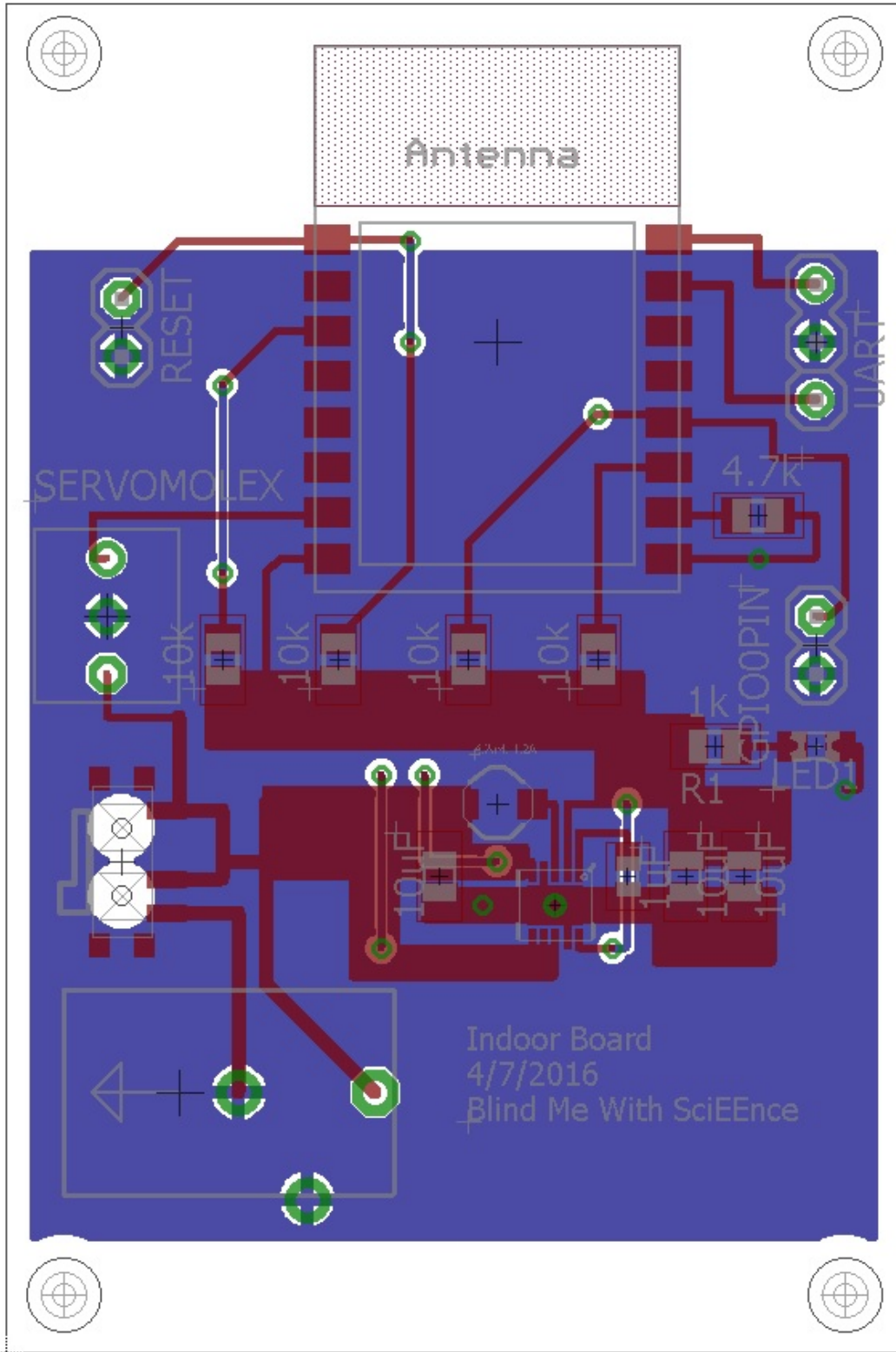
Figure 2. Indoor Board Layout
